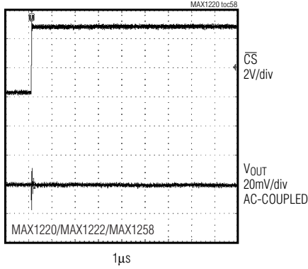
MAJOR CARRY TRANSITION RLOAD = 10kΩ, CLOAD = 100pF
